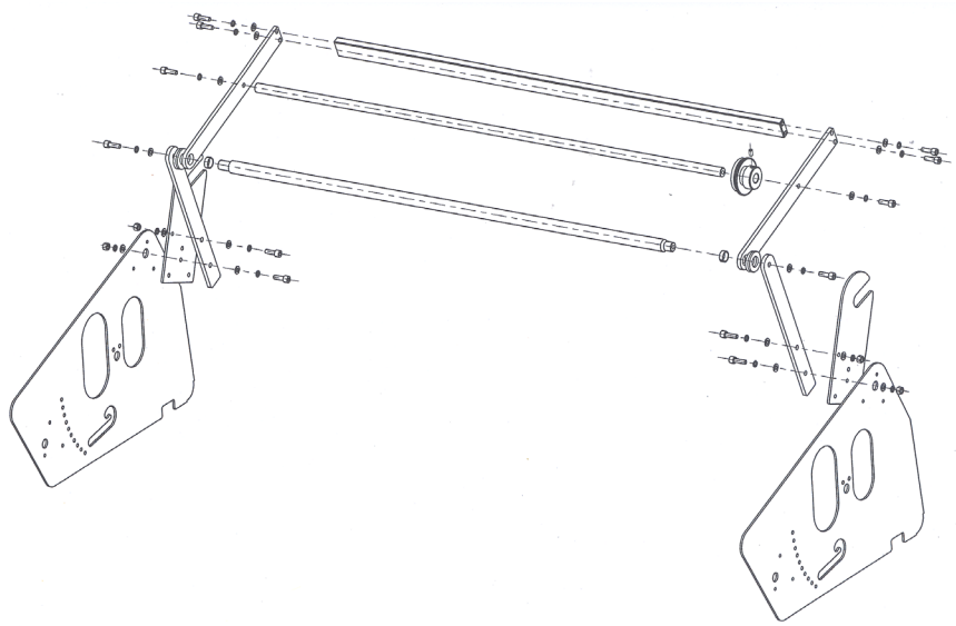
Optional Perforator assembly
